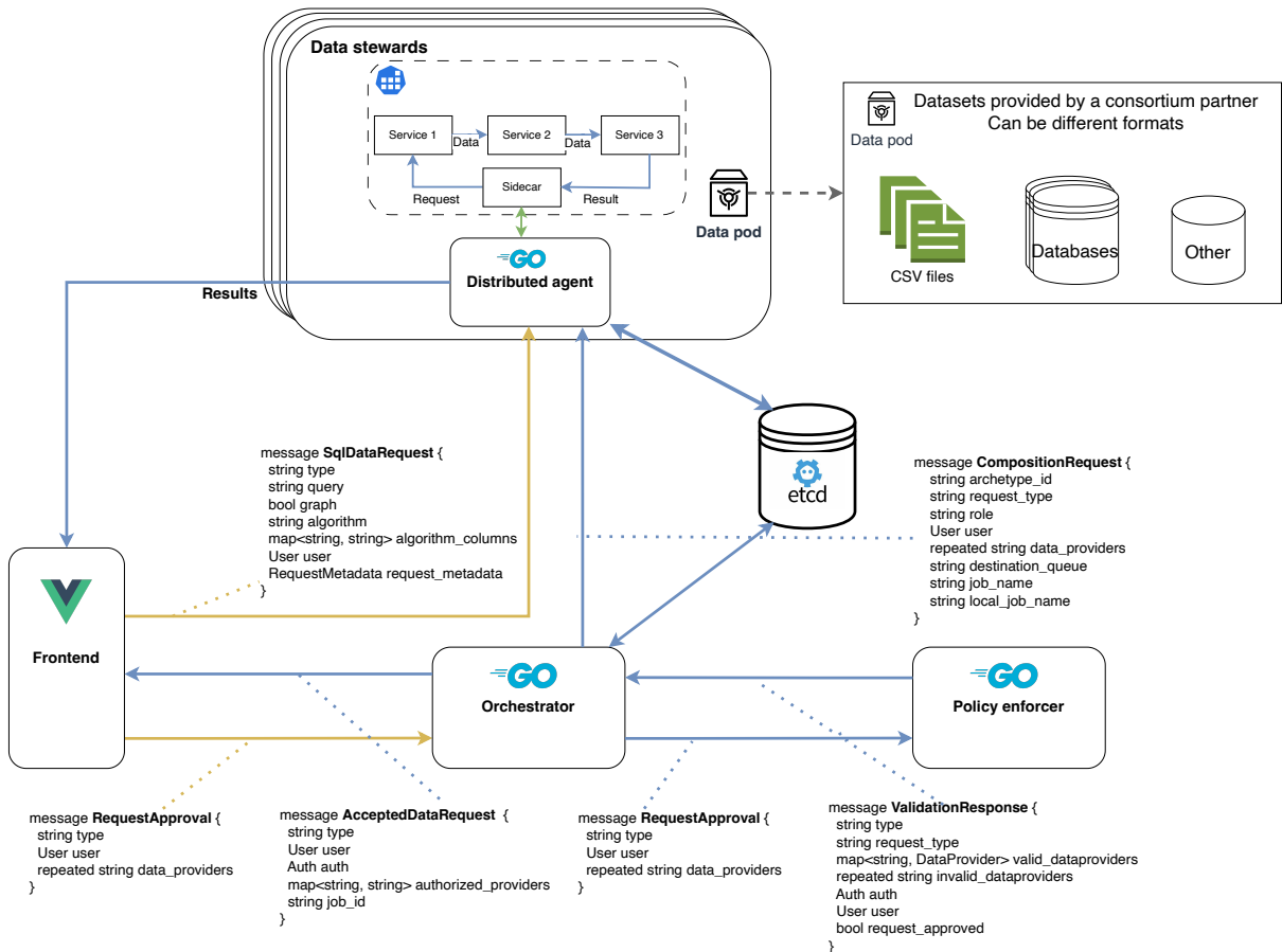
Figure 4.2: DYNAMOS architecture
